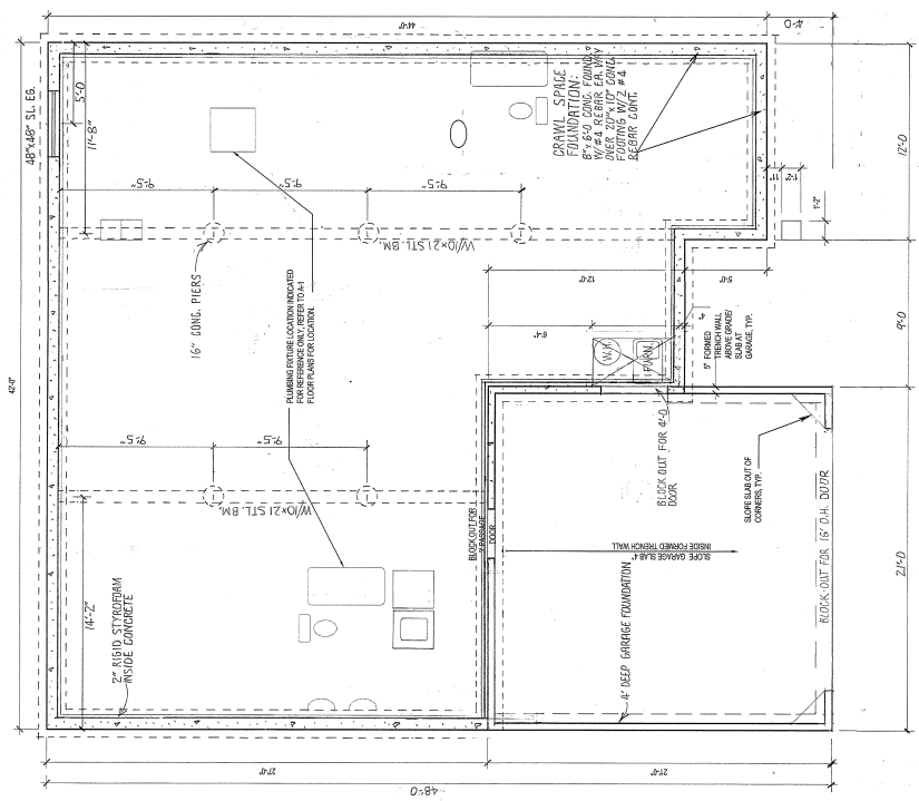
B Foundation Plan SCALE: 1/4" = 1'-0" 1/8" = 1'-0"
