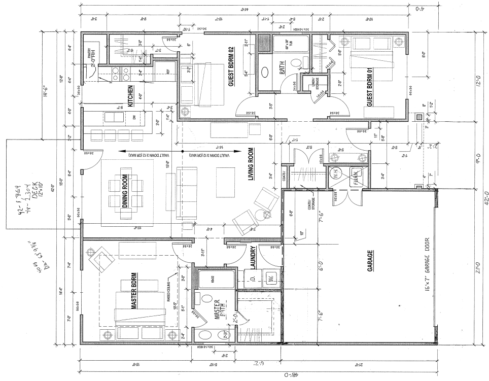
A Floor Plan SCALE: 1/4" = 1'-0" 1/8" = 1'-0"
